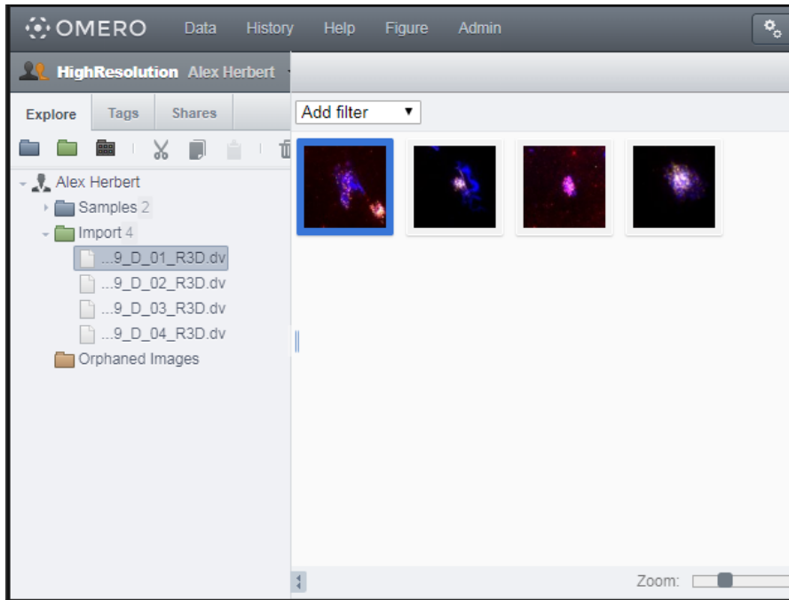
OMERO Client
