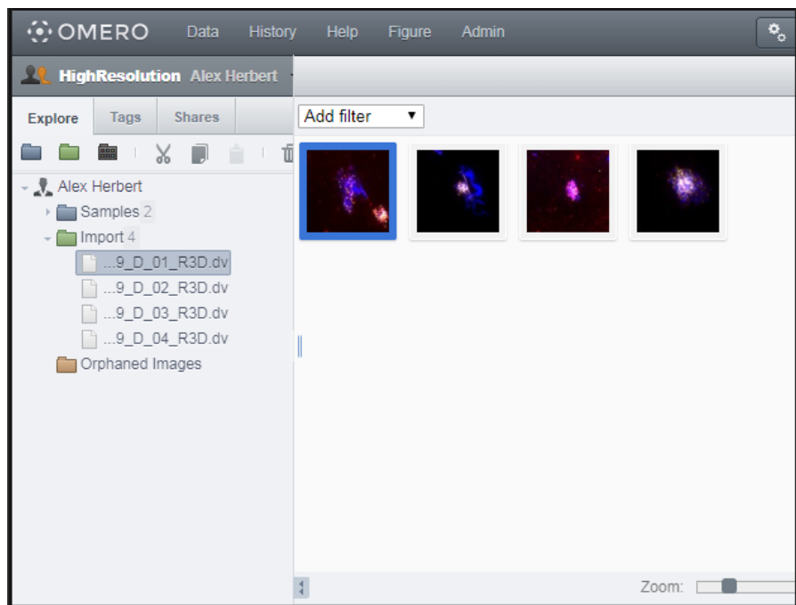
OMERO Client
